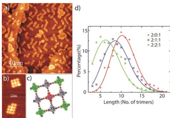
Figure 4. (a) STM image of a mixture of 1 , 2 , and 3 (ratio 2:2:1) showing the appearance of shorter triple-strand ladders. (b,c) High-resolution image of the 3×3 squares and corresponding molecular model ( 1 , gray; 2 , green; and 3 , pink). (d) Length distribution of the triple-strand ladders (ratio 1:3 is set to 2:1) formed at different mixing ratios (values shown indicate mixing ratio of 1 , 2 , and 3 ) with Poisson fits.
