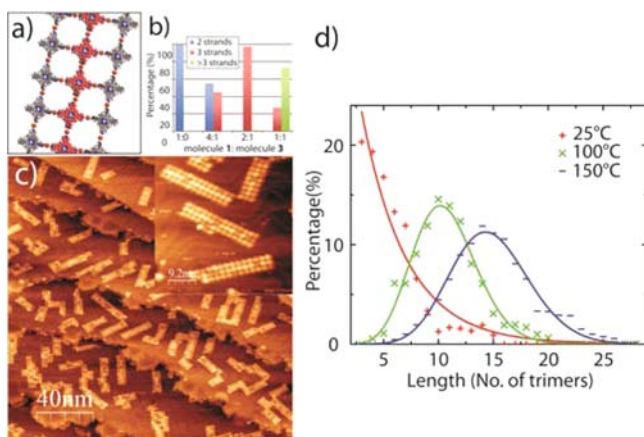
Figure 3. (a) Molecular model of the triple-strand ladder structure formed by 1 (gray) and 3 (pink). (b) Width distribution of the ladders at different ratios of 1 and 3 . (c) STM image of a 2:1 mixture of 1 and 3 , showing unique formation of the triple-strand ladders; inset, a high-resolution ( 40 \times 40 \text{ nm}^2 ) image of the triple-strand ladders. (d) Length distribution of the triple-strand ladders grown at 25 (red), 100 (green), and 150 °C (blue) with Flory–Schulz and Poisson fits.
