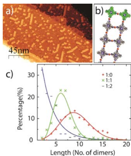
Figure 2. (a) STM image of a sample with 1 and 2 mixed in a ratio of 1:2 after annealing at 100 °C. (b) Model of a ladder end with 2 acting as a molecular stopper (in green). (c) Length distribution of the double-strand ladders formed at different mixing ratios (values shown indicate mixing ratio of 1 and 2 ) with Flory–Schulz and Poisson fits.
