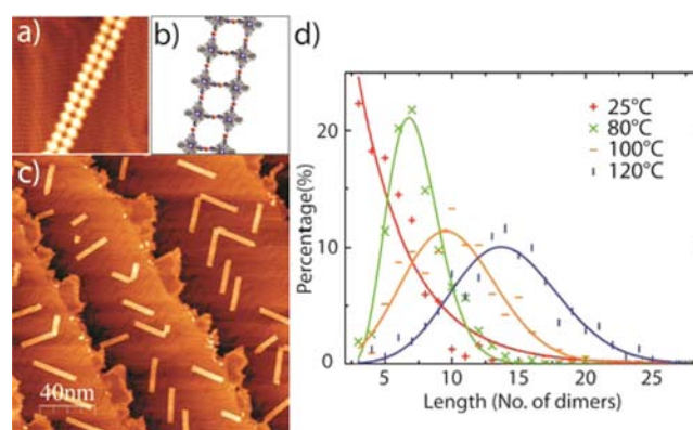
Figure 1. (a) High-resolution STM image ( 20 \times 20 \text{ nm}^2 ) of the double-strand ladder structure formed by 1 and Cu. (b) Corresponding molecular model of the double-strand ladder structure. (c) STM image of the sample after annealing at 120 \text{ }^\circ\text{C} . (d) Length distributions of the sample after annealing at 25 (red), 80 (green), 100 (orange), and 120 \text{ }^\circ\text{C} (blue) with Flory–Schulz and Poisson fits.
